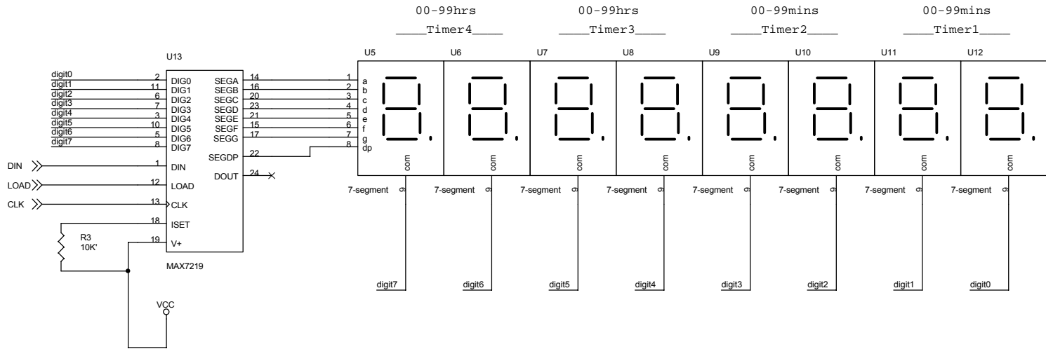
U6-U12 are common cathode 7-segment LEDs
