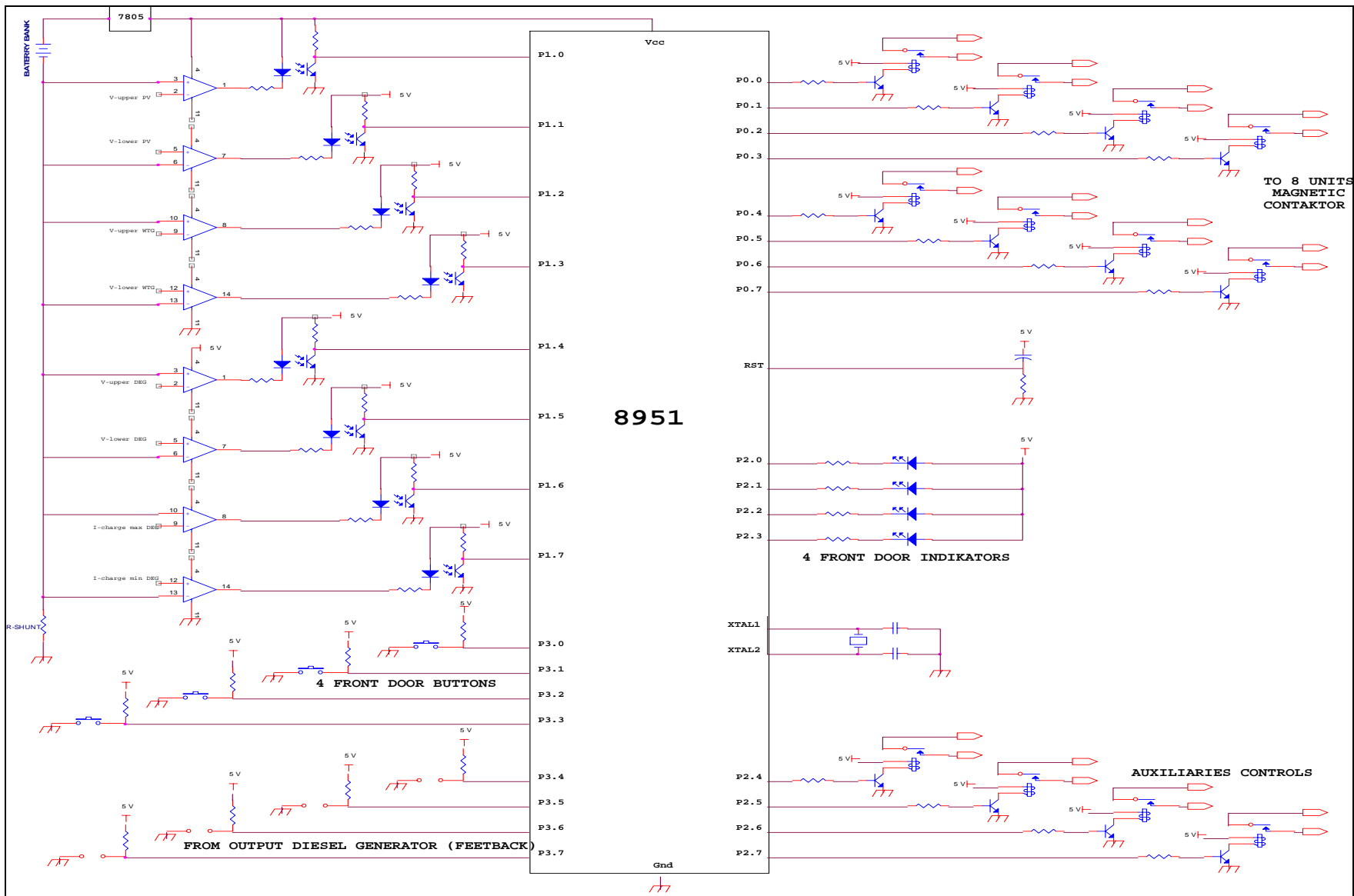
Figure 4. Controller's schematic
